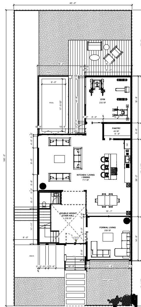
BACK SIDE
